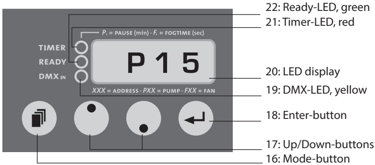
Abb. 1: Display shown at adjusting the pump output
