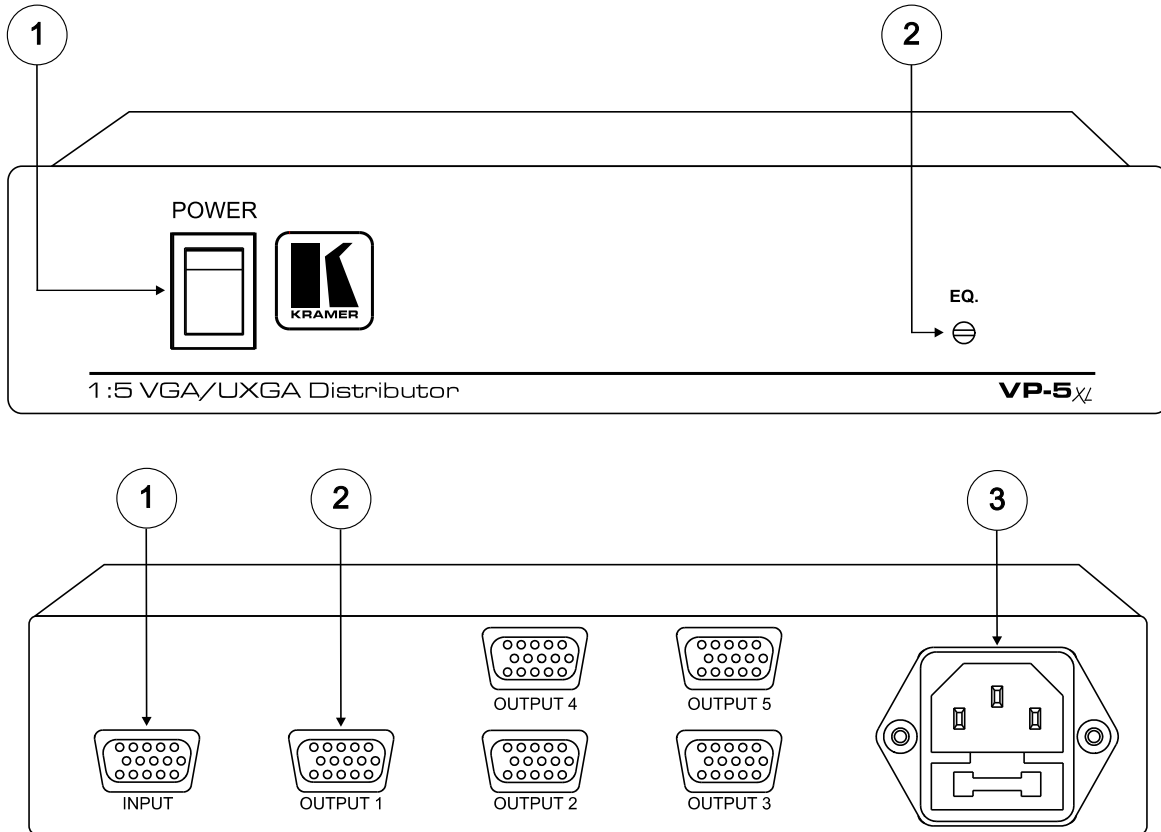
Figure 3: VP-5xl 1:5 VGA/UXGA Distributor
