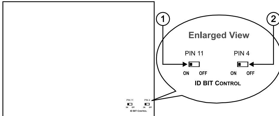
Figure 4: VGA/UXGA Distributor Underside
