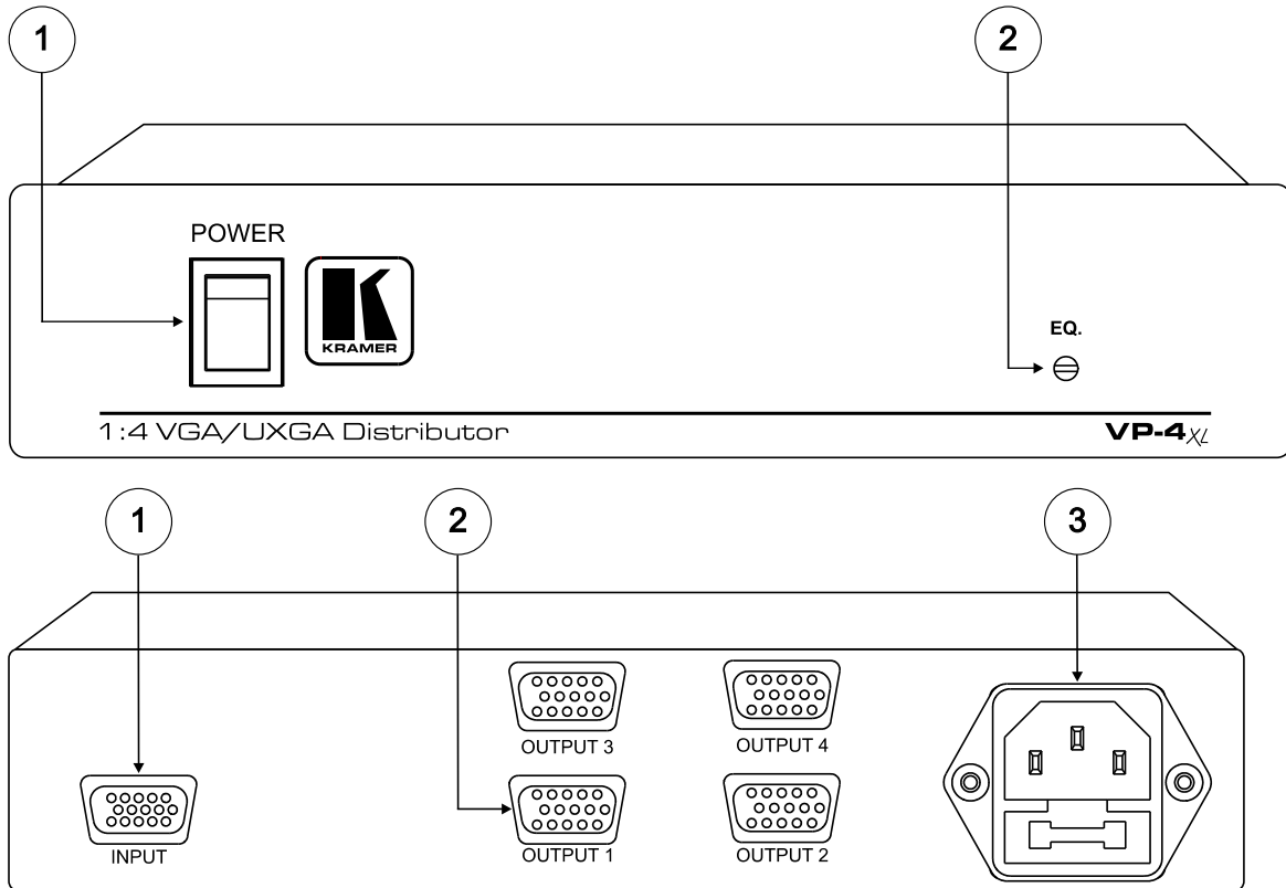
Figure 2: VP-4xl 1:4 VGA/UXGA Distributor
